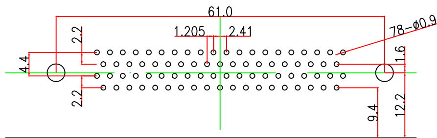
PCB LAYOUT
