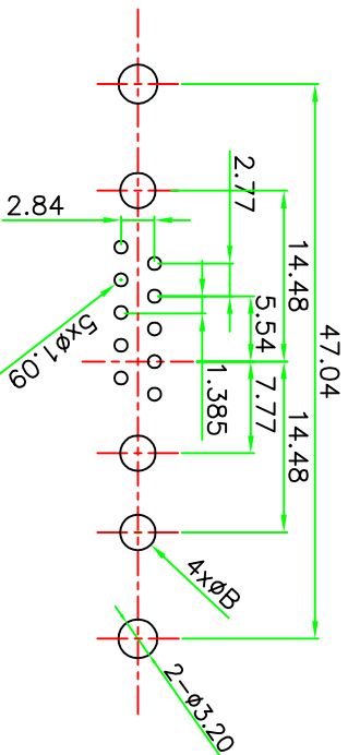
PCB LAYOUT
